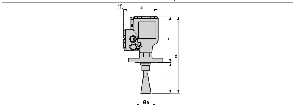
Figure 2-10: Metallic Horn antennas with standard flange connections
