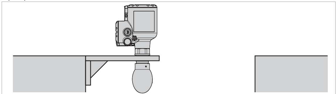
Figure 3-9: Open pits
