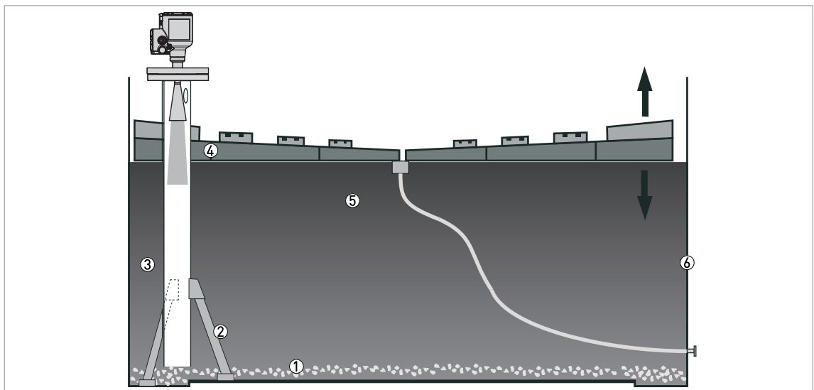
Figure 3-11: Floating roofs
