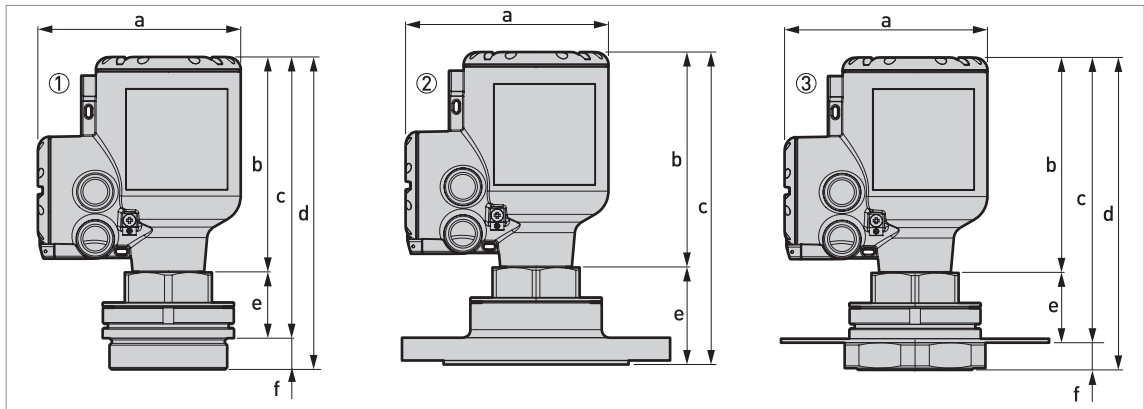
Figure 2-18: DN70 / 2 \frac{3}{4} " Lens antenna versions
